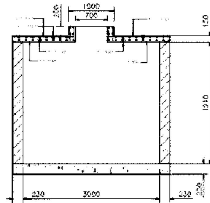
SECTION C-C SCALE 1/4"
