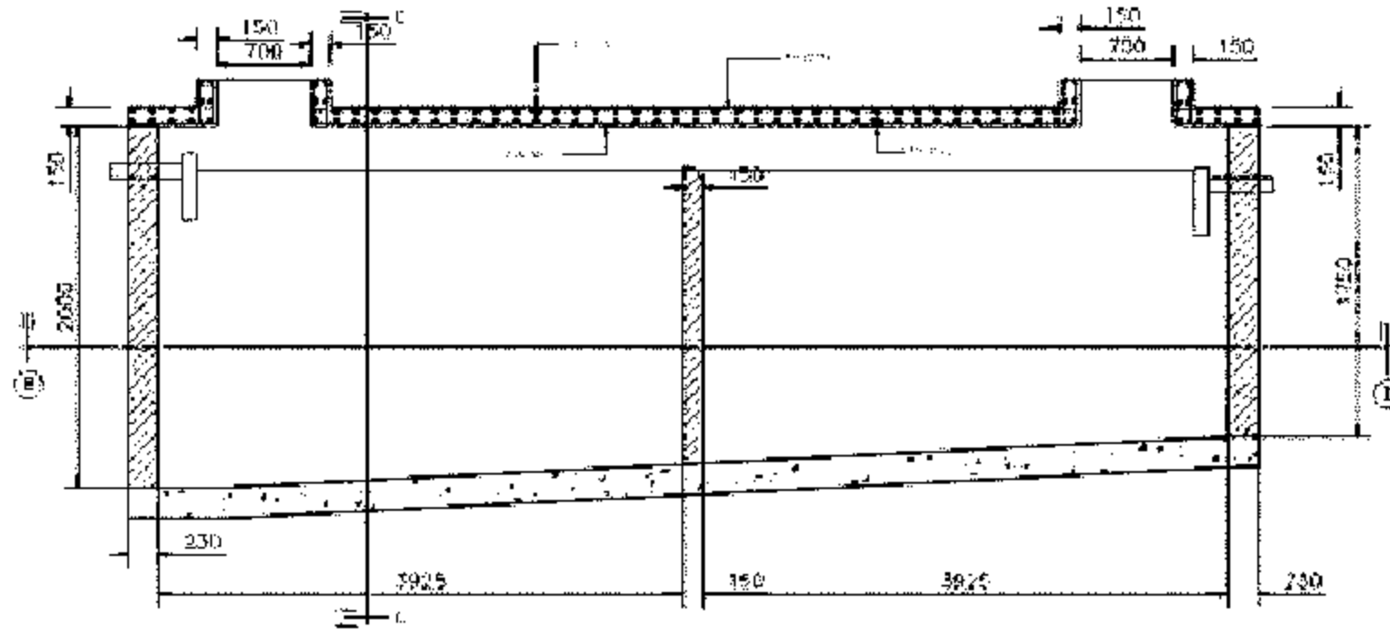
SECTION A-A SCALE 1/4"
